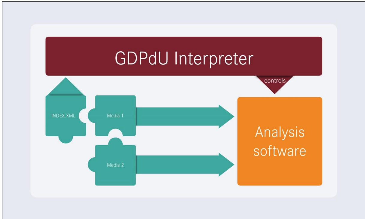
Figure 4: Import process
